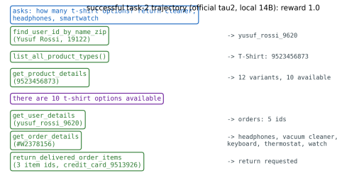
Figure 3: A successful task-2 trajectory on the official tau2 retail environment (local Qwen2.5-14B): the agent finds the user, counts the 10 available t-shirt variants, communicates the count, locates the items, and executes the three-item return with real ids. The hidden evaluator scores DB 1.0 and NL-assertion 1.0.
