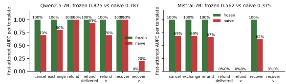
Figure 4: F3 mechanism: per-template first-attempt AUPC, frozen vs. naive. On both backbones the degradation concentrates on the templates the frozen policy solved, while never-solved templates stay flat (and on Qwen the hardest variant even improves +0.2 ). The update suppresses the action patterns it trained on with mixed credit.
