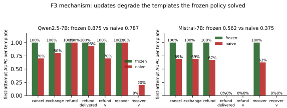
Figure 5: F3 mechanism: per-template first-attempt AUPC, frozen vs. naive. On both backbones the degradation concentrates on the templates the frozen policy solved, while never-solved templates stay flat (and on Qwen the hardest variant even improves +0.2 ). The update suppresses the action patterns it trained on with mixed credit.
