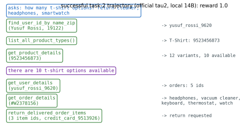
Figure 6: A successful task-2 trajectory on the official tau2 retail environment (local Qwen2.5-14B): the agent finds the user, counts the 10 available t-shirt variants, communicates the count, locates the items, and executes the three-item return with real ids. The hidden evaluator scores DB 1.0 and NL-assertion 1.0.
