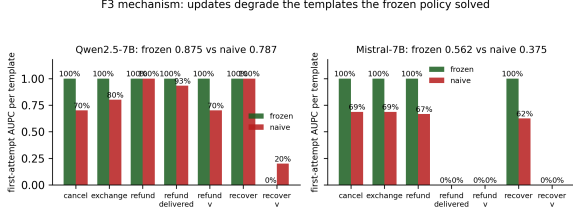
Figure 4: F3 mechanism: per-template first-attempt AUPC, frozen vs. naive. On both backbones the degradation concentrates on the templates the frozen policy solved, while never-solved templates stay flat (and on Qwen the hardest variant even improves +0.2). The update suppresses the action patterns it trained on with mixed credit.
