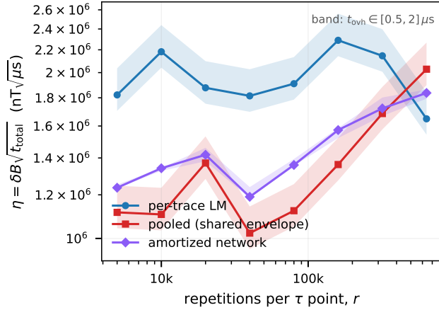
FIG. 3. Sensitivity \eta = \delta B \sqrt{t_{\text{total}}} against repetitions per delay point for per-trace and pooled inference, with the per-point overhead t_{\text{ovh}} varied over 0.5 , 1 and 2 \mu s . The crossover is overhead-independent.
