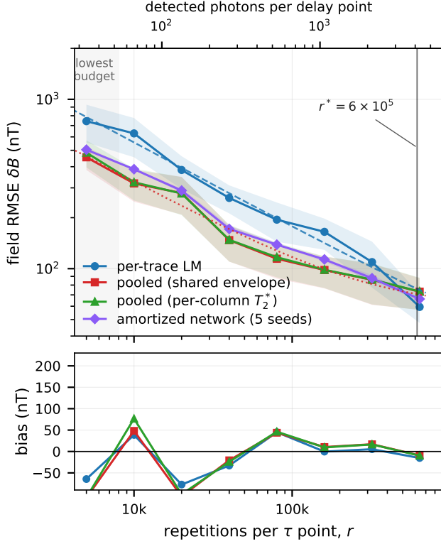
FIG. 1. Real data, columns 7–40. Top: field RMSE against repetitions per delay point for the four estimators. Shaded bands are variability , not confidence intervals: for the classical estimators they span the column-to-column interquartile range within the single measured session, for the network the range across the five training seeds (hatched). The columns are field settings, not independent experimental replications, so the bands describe how consistent an ordering is across fields, not a sampling uncertainty of the method. Dashed and dotted curves are the two-term law of Eq. (2) fitted to the per-trace and pooled ladders; the vertical line is the crossover r^* . Bottom: signed mean error of the same estimators on the same traces (symmetric-log scale). The crossover in the top panel is the point where the pooled estimators’ growing bias, visible in the bottom panel, overtakes their bound advantage. The shaded strip marks the lowest measured budget.
