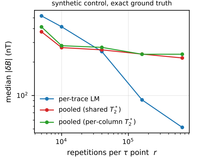
FIG. 3. Synthetic control with exact ground truth and the measured envelope population. Median field error against budget for per-trace fitting, full pooling and partial pooling. Note the reversal between the lowest and the highest budgets.
