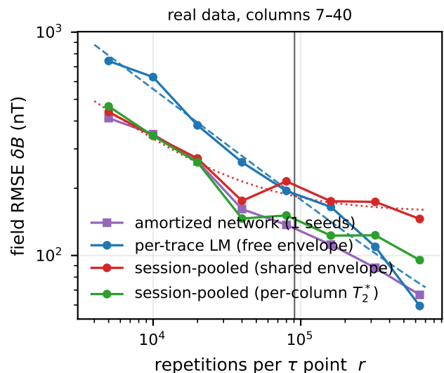
FIG. 1. Field RMSE against repetitions per delay point, real data, columns 7–40. Markers are the measured estimators; dashed and dotted lines are the two-term law of Eq. (2) fitted to the per-trace and pooled ladders. The vertical line marks the crossover r^* .
