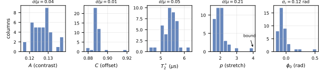
FIG. 4. Relaxation envelope measured across the 40 field settings from the highest-budget sheet. The phase \phi_0 is essentially common (circular concentration \geq 0.99 ), whereas the relaxation time varies by \pm 5\% ; that inhomogeneity sets the pooled bias floor.
