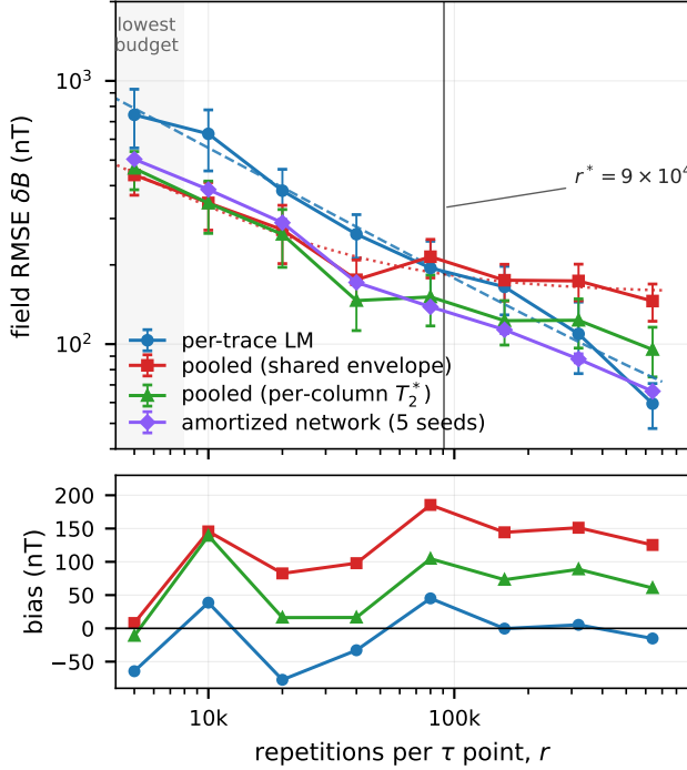
FIG. 1. Real data, columns 7–40. Top: field RMSE against repetitions per delay point for the four estimators; error bars are percentile bootstrap intervals over the 34 columns (for the network, the interquartile spread over training seeds). Dashed and dotted curves are the two-term law of Eq. (2) fitted to the per-trace and pooled ladders; the vertical line is the crossover r^* . Bottom: signed mean error of the same estimators on the same traces (symmetric-log scale). The crossover in the top panel is the point where the pooled estimators’ growing bias, visible in the bottom panel, overtakes their bound advantage. The shaded strip marks the lowest measured budget.
