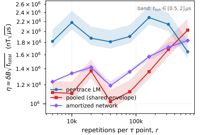
FIG. 3. Sensitivity \eta = \delta B \sqrt{t_{\text{total}}} against repetitions per delay point for per-trace and pooled inference, with the per-point overhead t_{\text{ovh}} varied over 0.5, 1 and 2 \mu\text{s} . The crossover is overhead-independent.
