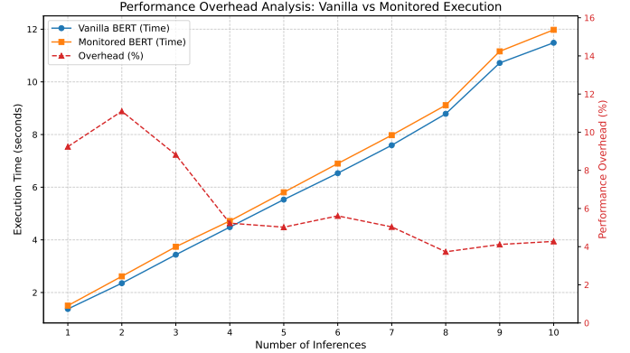
Fig. 3: Performance overhead analysis showing the execution time of Vanilla vs. Monitored BERT and the relative overhead percentage across varying numbers of inferences.
