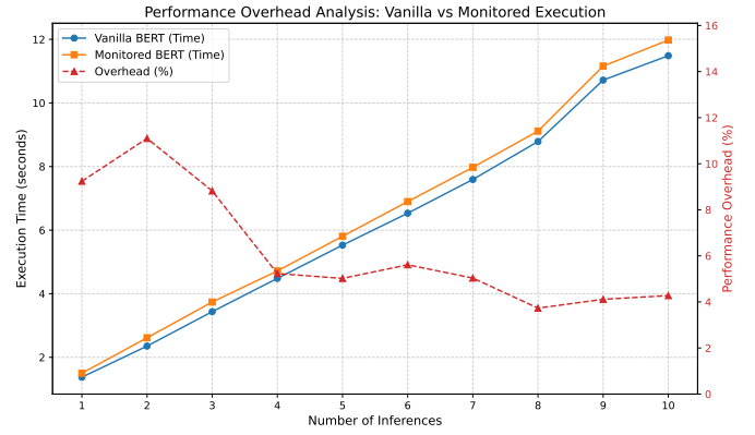
Fig. 3: Performance overhead analysis showing the execution time of Vanilla vs. Monitored BERT and the relative overhead percentage across varying numbers of inferences.
