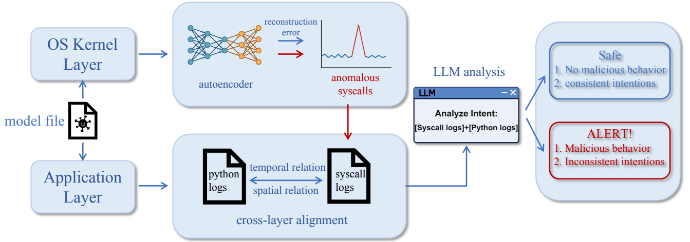
Fig. 3: Overview of the hybrid defense system.
