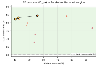
Figure 17: RF ( f1_{pa} ) on scene : Pareto frontier of (abstention, retained quality) with the win-region shaded green (left); per-method per-noise gain ( f1_{pa} - f1 ) heatmap (right).
