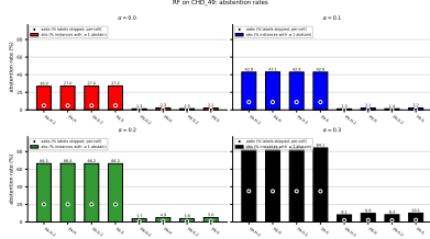
Figure 31: RF (f1_pa) on CHD_49: abstention rates (left) and standard-MLC-vs-abstention paired bars (right), across \alpha \in \{0.0, 0.1, 0.2, 0.3\} . Left: bar = abs (% of instances with at least one abstained label, instance-level); dot = aabs (% of labels skipped, per-cell label-level). These rates are independent of the quality metric. Right: blue = standard MLC quality (no abstention) on the matched BV metric; coloured = with-abstention quality on retained labels.
