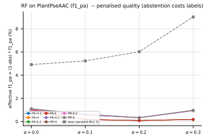
Figure 22: RF ( f1_{pa} ) on PlantPseAAC — robustness view. Left: efficiency-quality scatter ( x = \text{coverage} = 1 - \text{abs} ); upper-right is robust (predicts many labels and keeps quality high). Right: effective f1_{pa} = (1 - \text{abs}) \cdot f1_{pa} , i.e. retained quality penalised by skipped coverage. A method whose effective curve stays above the dashed standard-MLC baseline at every \alpha is robust to noise, not just selectively abstaining on hard labels.
