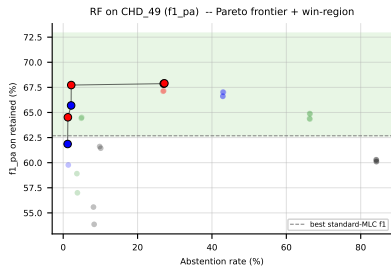
Figure 33: RF (f1_pa) on CHD_49: Pareto frontier of (abstention, retained quality) with the win-region shaded green (left); per-method per-noise gain ( f1_{pa} - f1 , percentage points) heatmap (right).
