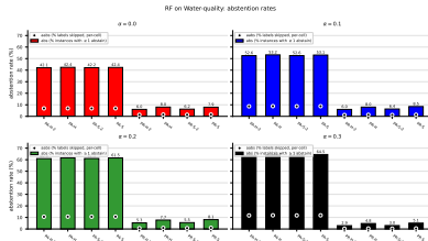
Figure 35: RF (f1 pa ) on Water-quality: abstention rates (left) and standard-MLC-vs-abstention paired bars (right), across \alpha \in \{0.0, 0.1, 0.2, 0.3\} . Left: bar = abs (% of instances with at least one abstained label, instance-level); dot = aabs (% of labels skipped, per-cell label-level). These rates are independent of the quality metric. Right: blue = standard MLC quality (no abstention) on the matched BV metric; coloured = with-abstention quality on retained labels.
