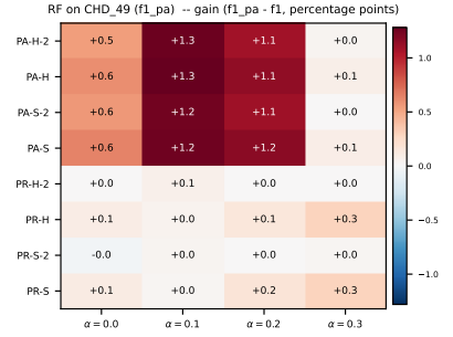
Figure 33: RF (f1_pa) on CHD_49: Pareto frontier of (abstention, retained quality) with the win-region shaded green (left); per-method per-noise gain ( f1_{pa} - f1 , percentage points) heatmap (right).
