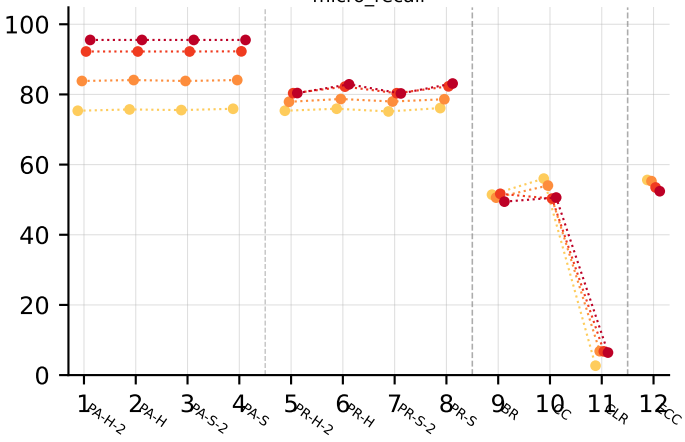
micro_recall
