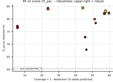
Figure 18: RF ( f1_{pa} ) on scene — robustness view. Left: efficiency-quality scatter ( x = \text{coverage} = 1 - \text{abs} ); upper-right is robust (predicts many labels and keeps quality high). Right: effective f1_{pa} = (1 - \text{abs}) \cdot f1_{pa} , i.e. retained quality penalised by skipped coverage. A method whose effective curve stays above the dashed standard-MLC baseline at every \alpha is robust to noise, not just selectively abstaining on hard labels.
