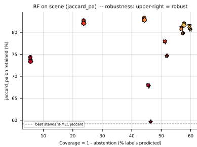
Figure 58: RF (jaccard pa ) on scene — robustness view. Left: efficiency-quality scatter (x = coverage = 1 − abs); upper-right is robust (predicts many labels and keeps quality high). Right: effective jaccard pa = (1 − abs) · jaccard pa , i.e. retained quality penalised by skipped coverage. A method whose effective curve stays above the dashed standard-MLC baseline at every \alpha is robust to noise, not just selectively abstaining on hard labels.
