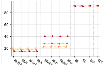
f_{MLC}^{ham} (??) ( \uparrow )
