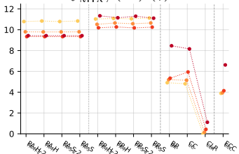
f_{MLC}^{Jacc} (??) ( \uparrow )
