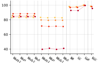
AFRD (??) ( \downarrow )
