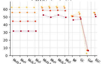
f_{MLC}^{Jacc} (??) ( \uparrow )
