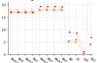
f_{MLC}^1 (??) ( \uparrow )
