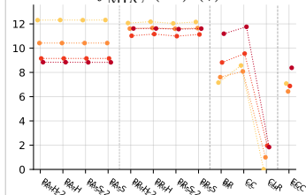
f_{MLC}^{Jacc} (??) ( \uparrow )
