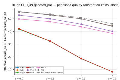
Figure 74: RF (jaccard.pa) on CHD_49 — robustness view. Left: efficiency-quality scatter ( x = coverage = 1 - abs ); upper-right is robust (predicts many labels and keeps quality high). Right: effective jaccard.pa = (1 - abs) \cdot jaccard.pa , i.e. retained quality penalised by skipped coverage. A method whose effective curve stays above the dashed standard-MLC baseline at every \alpha is robust to noise, not just selectively abstaining on hard labels.
