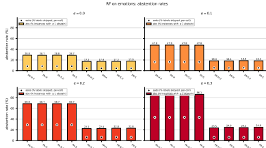
Figure 11: RF (f1_pa) on emotions: abstention rates (left) and standard-MLC-vs-abstention paired bars (right), across \alpha \in \{0.0, 0.1, 0.2, 0.3\} . Left: bar = abs (% of instances with at least one abstained label, instance-level); dot = aabs (% of labels skipped, per-cell label-level). These rates are independent of the quality metric. Right: blue = standard MLC quality (no abstention) on the matched BV metric; coloured = with-abstention quality on retained labels.
