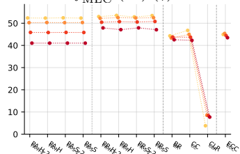
macro- f_1 (??) ( \uparrow )
