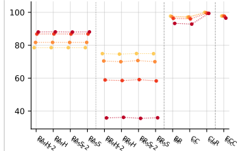
AFRD (??) ( \downarrow )
