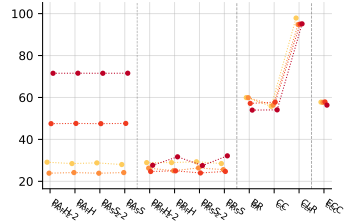
AFRD (??) ( \downarrow )
