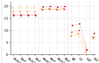
f_{MLC}^1 (??) ( \uparrow )
