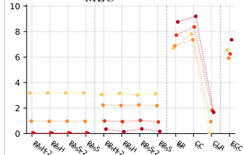
f_{MLC}^{sub} (??) ( \uparrow )
