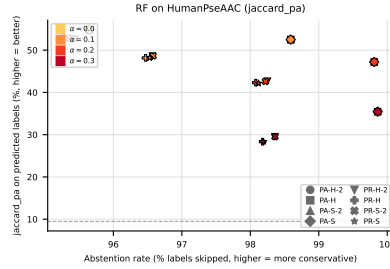
Figure 64: RF (jaccard_pa) on HumanPseAAC : coverage-risk scatter. Each point is one (method, noise) pair; x = abstention rate, y = quality on retained labels. Points above the dashed line beat the best standard-MLC baseline.
