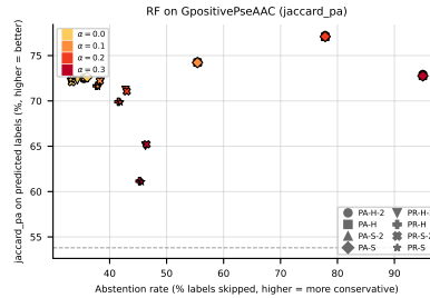
Figure 48: RF (jaccard pa ) on GpositivePseAAC: coverage-risk scatter. Each point is one (method, noise) pair; x = abstention rate, y = quality on retained labels. Points above the dashed line beat the best standard-MLC baseline.
