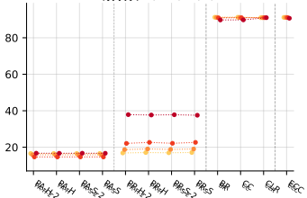
f_{MLC}^{ham} (??) ( \uparrow )
