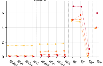
f_{MLC}^{sub} (??) ( \uparrow )
