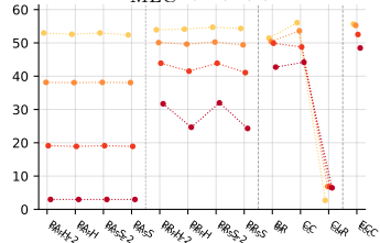
f_{MLC}^{sub} (??) ( \uparrow )
