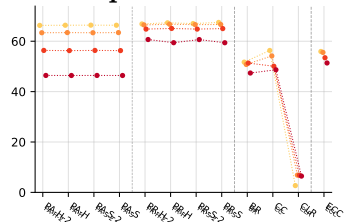
f_{MLC}^1 (??) ( \uparrow )
