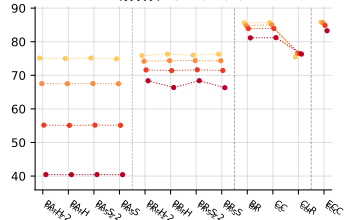
f_{MLC}^{ham} (??) ( \uparrow )
