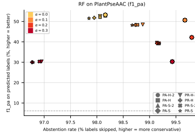
Figure 20: RF ( f1_{pa} ) on PlantPseAAC : coverage-risk scatter. Each point is one (method, noise) pair; x = \text{abstention rate} , y = \text{quality on retained labels} . Points above the dashed line beat the best standard-MLC baseline.
