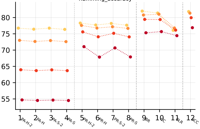
hamming_accuracy
