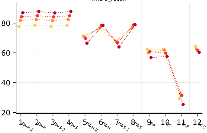
micro_recall
