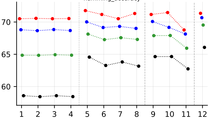
hamming_accuracy
