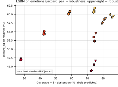
Figure 132: LGBM ( jaccard\_pa ) on emotions — robustness view. Left: efficiency-quality scatter ( x = coverage = 1 - abs ); upper-right is robust (predicts many labels and keeps quality high). Right: effective jaccard\_pa = (1 - abs) \cdot jaccard\_pa , i.e. retained quality penalised by skipped coverage. A method whose effective curve stays above the dashed standard-MLC baseline at every \alpha is robust to noise, not just selectively abstaining on hard labels.
