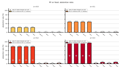
Figure 29: RF ( f1_{pa} ) on Yeast : abstention rates (left) and standard-MLC-vs-abstention paired bars (right), across \alpha \in \{0.0, 0.1, 0.2, 0.3\} . Left: bar = abs (% of instances with at least one abstained label, instance-level); dot = aabs (% of labels skipped, per-cell label-level). These rates are independent of the quality metric. Right: blue = standard MLC quality (no abstention) on the matched BV metric; coloured = with-abstention quality on retained labels.
