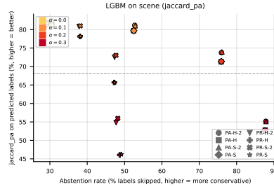
Figure 134: LGBM ( jaccard\_pa ) on scene : coverage-risk scatter. Each point is one (method, noise) pair; x = abstention rate, y = quality on retained labels. Points above the dashed line beat the best standard-MLC baseline.
