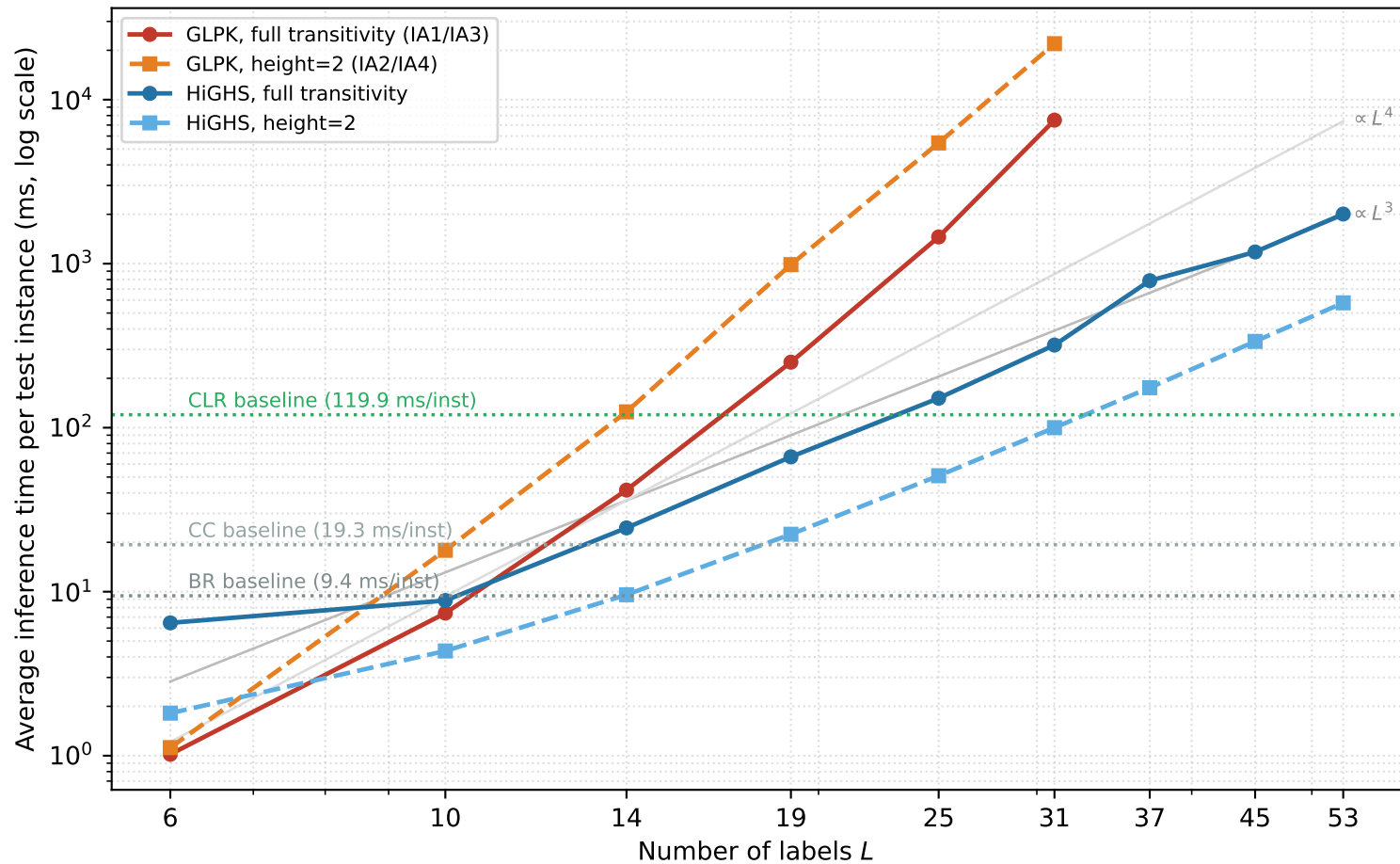
BOPOs ILP inference cost vs. label-set size (real enron RF pairwise probabilities, mean over 60 test instances)
