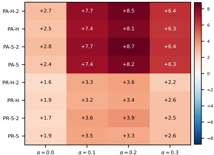
LGBM on emotions (jaccard_pa) -- gain (jaccard_pa - jaccard, percentage points)
