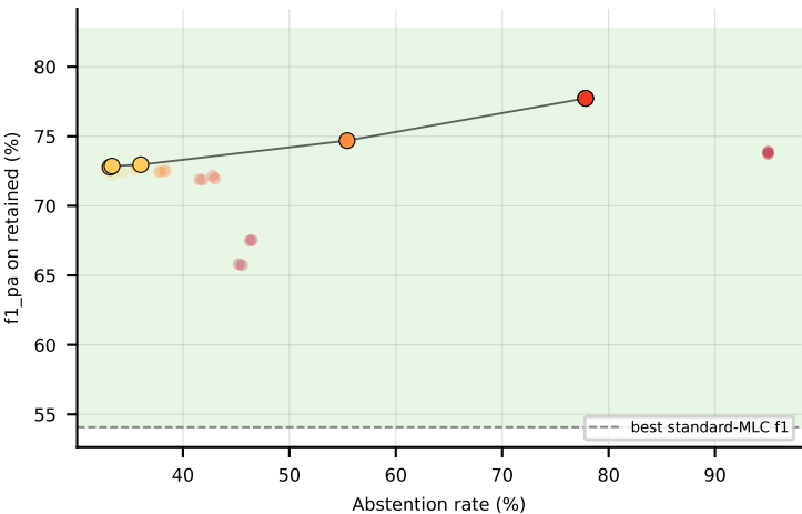
RF on GpositivePseAAC (f1_pa) -- Pareto frontier + win-region
