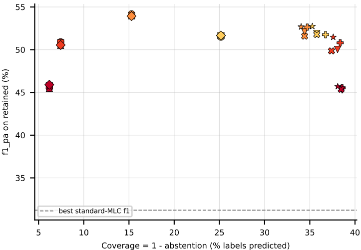
RF on VirusPseAAC (f1_pa) -- robustness: upper-right = robust
