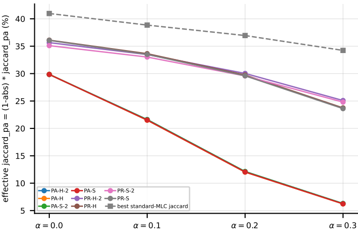
RF aggregate (jaccard_pa) -- penalised quality (abstention costs labels)
