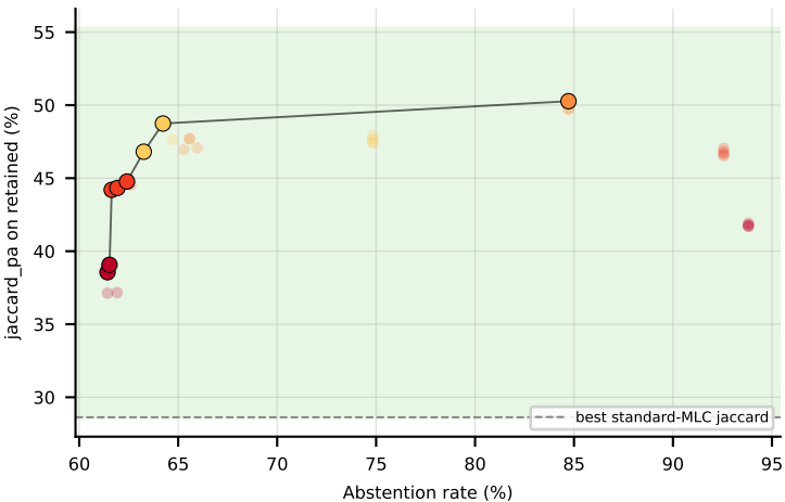
RF on VirusPseAAC (jaccard_pa) -- Pareto frontier + win-region
