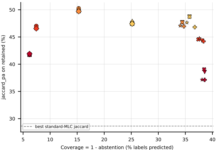
RF on VirusPseAAC (jaccard_pa) -- robustness: upper-right = robust
