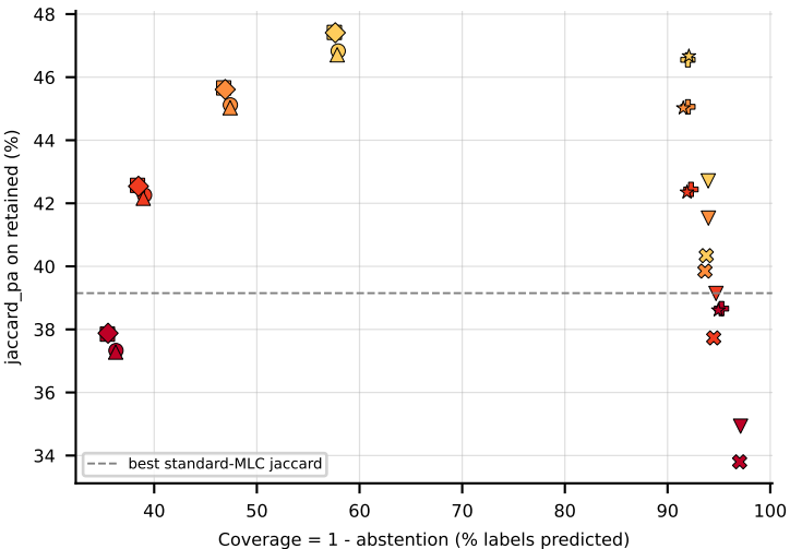
RF on Water-quality (jaccard_pa) -- robustness: upper-right = robust
