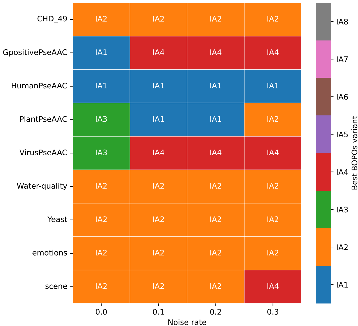
Best BOPOs variant per dataset × noise (hamming_accuracy)
