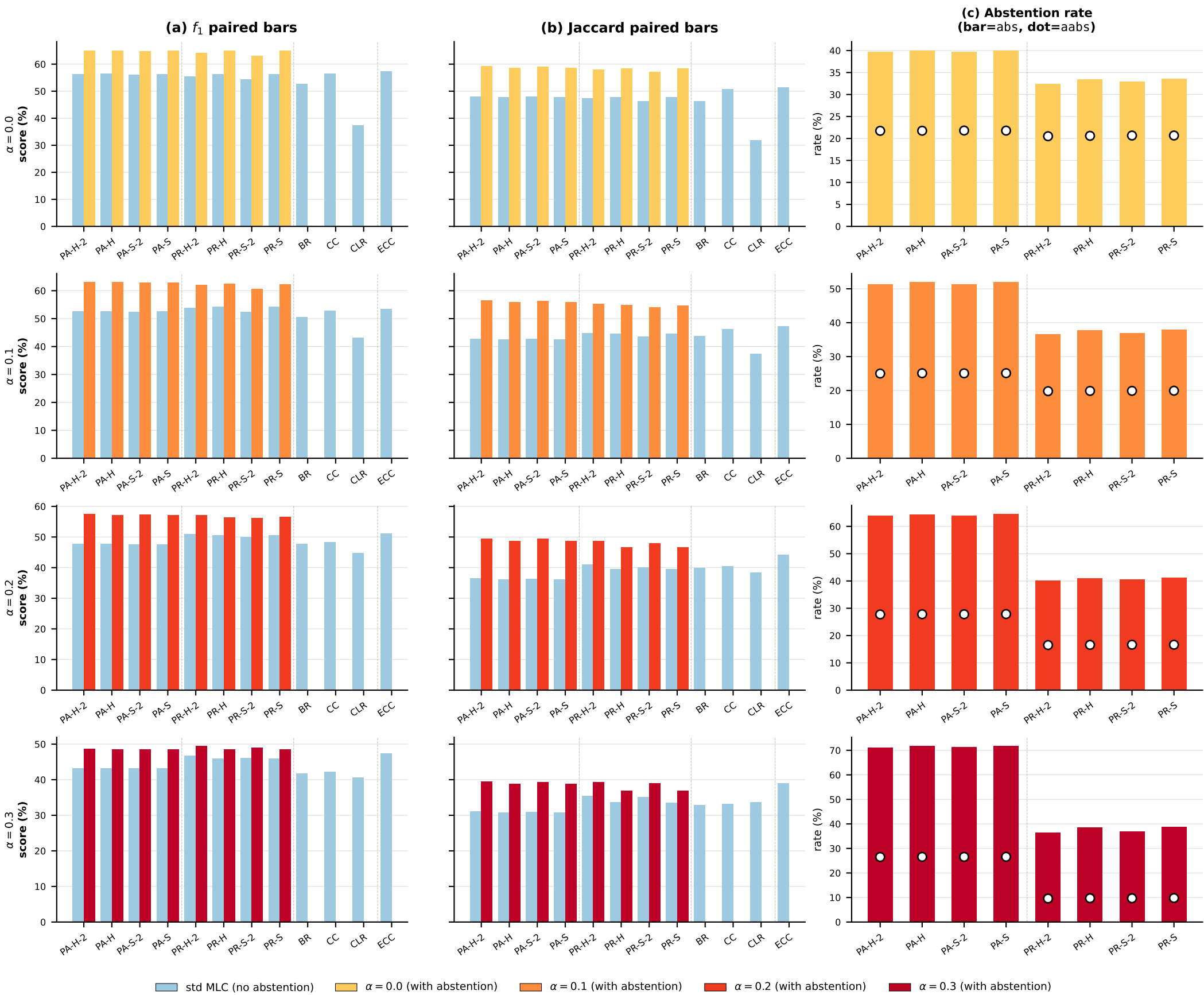
LGBM averaged across all datasets: abstention vs.\ standard MLC --- 4x3 grid (v1)
