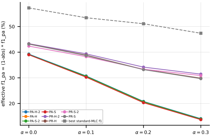
LGBM aggregate (f1_pa) -- penalised quality (abstention costs labels)
