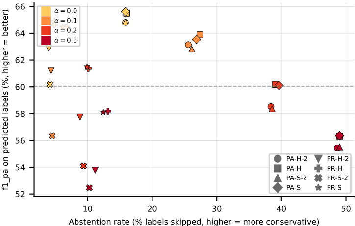
LGBM on CHD_49 (f1_pa)
