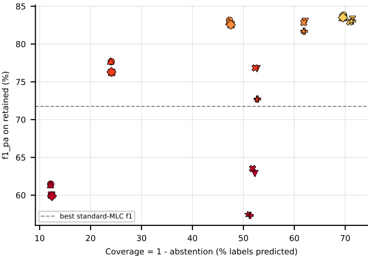
LGBM on scene (f1_pa) -- robustness: upper-right = robust
