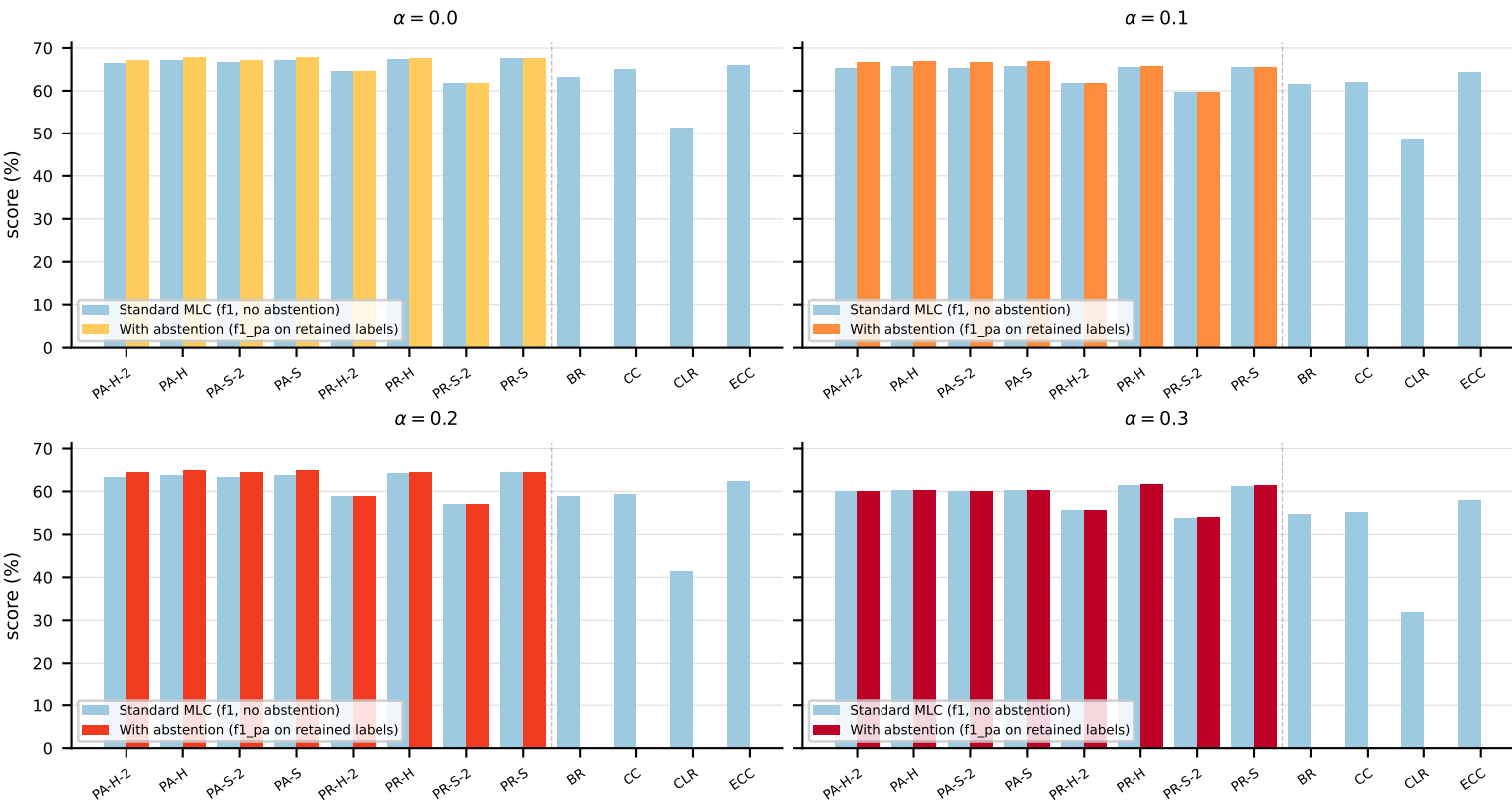
RF on CHD_49 (f1_pa)
