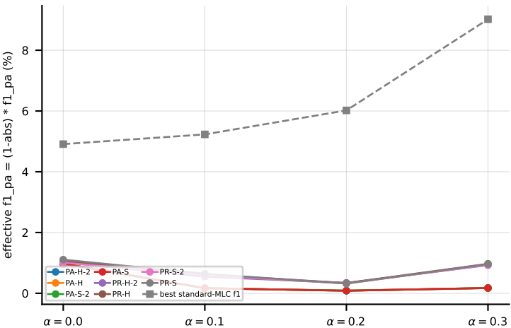
RF on PlantPseAAC (f1_pa) -- penalised quality (abstention costs labels)
