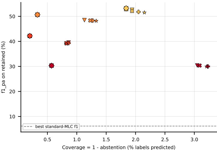
RF on PlantPseAAC (f1_pa) -- robustness: upper-right = robust
