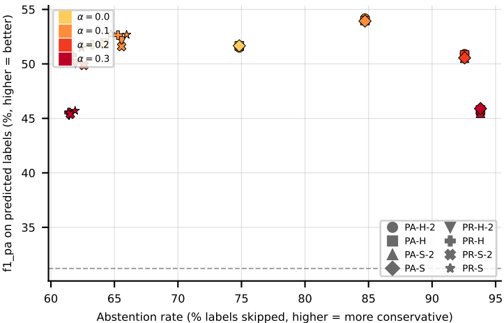
RF on VirusPseAAC (f1_pa)
