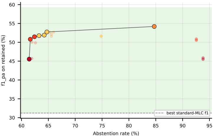
RF on VirusPseAAC (f1_pa) -- Pareto frontier + win-region
