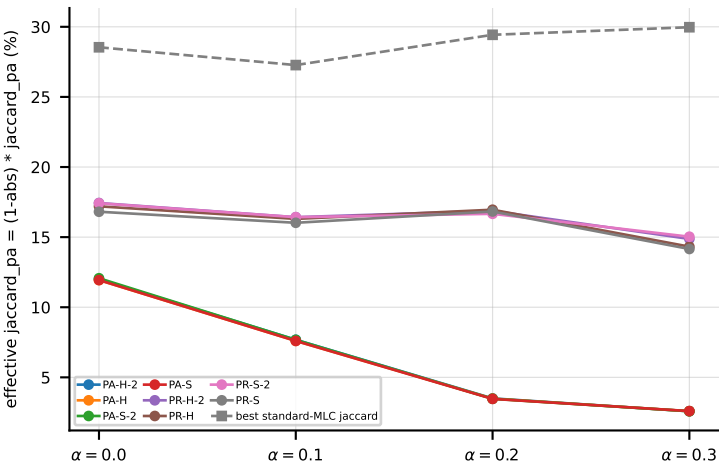
RF on VirusPseAAC (jaccard_pa) -- penalised quality (abstention costs labels)
