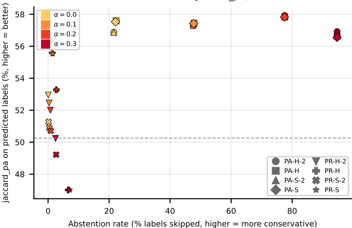
RF on Yeast (jaccard_pa)
