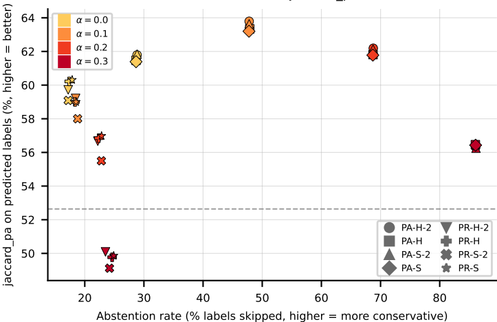
RF on emotions (jaccard_pa)
