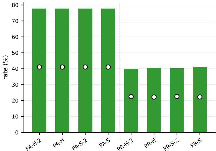
RF averaged across all datasets — Abstention rate \alpha = 0.2 (bar=abs, dot=aabs)
