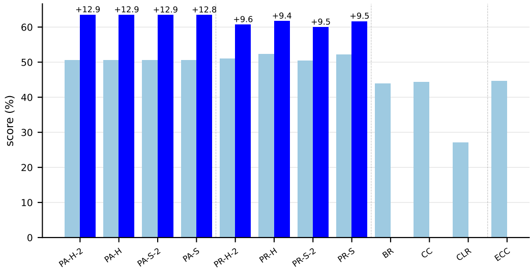
RF averaged across all datasets — f_1 paired bars \alpha = 0.1
