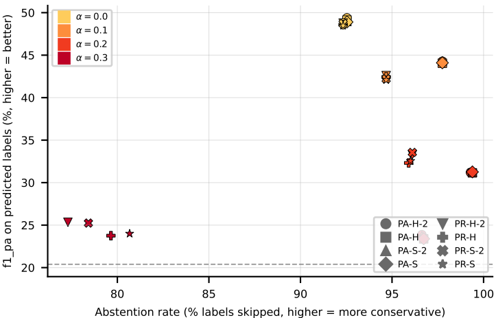
LGBM on PlantPseAAC (f1_pa)
