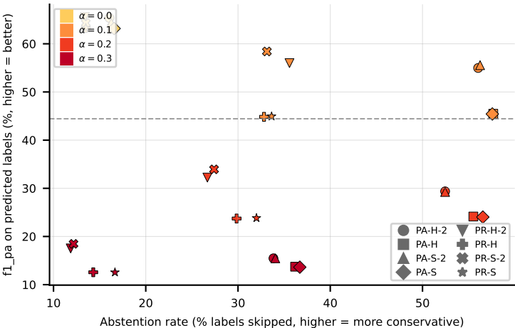
LGBM on medical (f1_pa)
