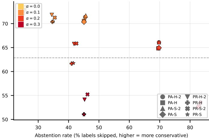
LGBM on GpositivePseAAC (jaccard_pa)
