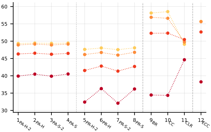
example_recall
