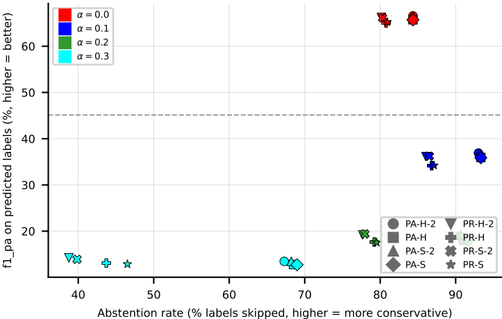
LGBM on birds (f1_pa)
