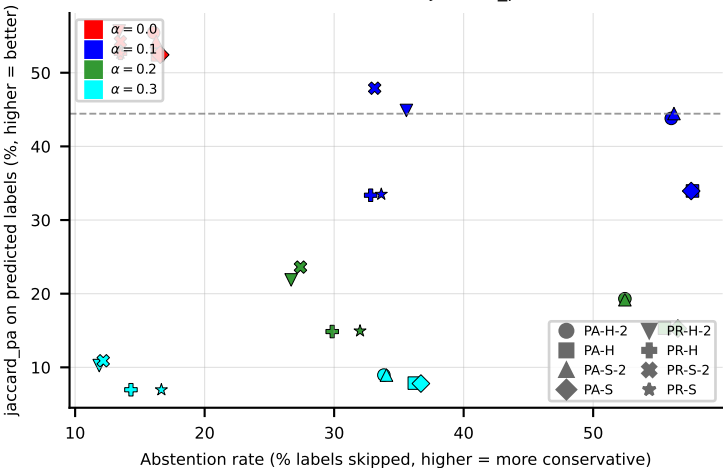
LGBM on medical (jaccard_pa)
