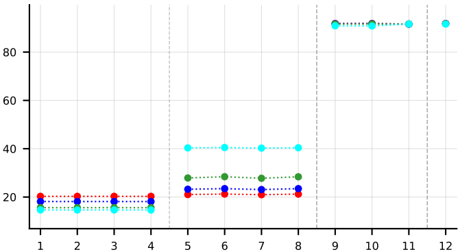
hamming_accuracy
