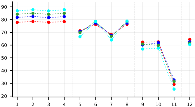
micro_recall
